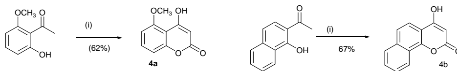
Scheme 3: Reaction scheme for the synthesis of derivatives of 4-hydroxycoumarin ( 4a and 4b ).
