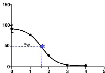
Fig 3: A sigmoid curve for the concentration-response plot of the enzyme assay.
