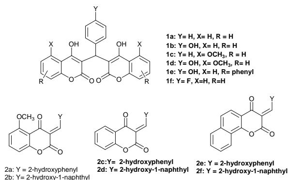
Fig 2: structures of the target compounds; symmetrical dimer ( 1a-f ) and asymmetrical ( 2a-f ) analogues of dicoumarol.
